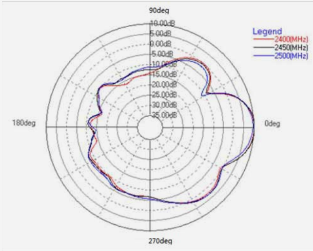
2.4G (PHI=0)
