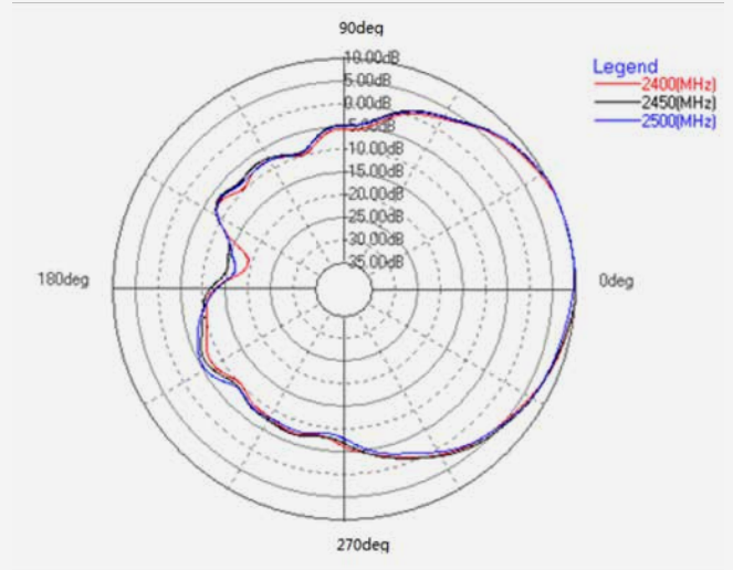
2.4G (PHI=90)
